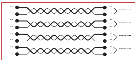
Split Pairs One pair uses one wire from another pair. The cable will work, but crosstalk may occur. Two or more pairs in the same cable may be split.
