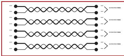
Open Pair One specific pair is open. It may be one or two wires in the same pair. One or more pairs may also be opened in the same cable.
