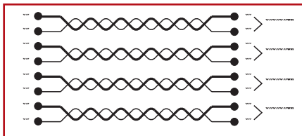
Crossed Pairs Two pairs are crossed at one end. Two or more pairs may be crossed in the same cable.
