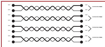
Shorted Wires Two wires from different pairs are shorted. Two or more wires and pairs may be affected in the same cable.
