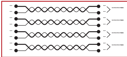
Crossed Wires Two wires from different pairs are crossed at one end. Two or more pairs may have wires crossed with another pair.
