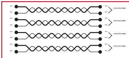
Reversed Pair The wires in one specific pair are reversed at one end. One or more pairs may be reversed in the same cable.
