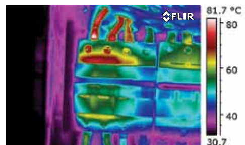
Overheated connection.
