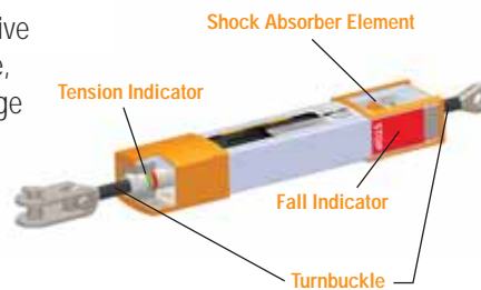
Turnbuckle
